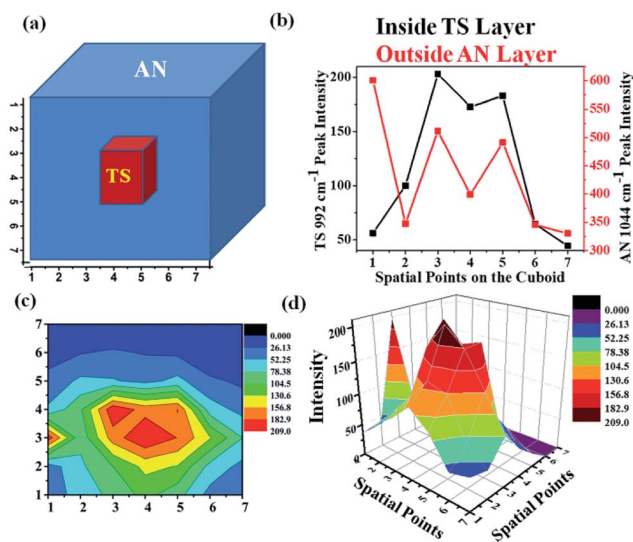
Fig. 11 Depth sensitive detection of bilayer solid powders ammonium nitrate (outer layer) and trans -stilbene (inner layer) using UMARS where, (a) depicts the bilayer cuboid sample schematically, (b) is the Raman intensity variation of AN & TS as the signals were collected by keeping the y-axis constant ( y = 4 ) i.e., at the center of the cuboid and by varying the x at that y, i.e., from x = 1 to x = 7 ; (c) shows the contour of the bilayer mapped with respect to TS Raman intensity where red colours corresponds to maximum TS intensity, blue corresponds to a minimum value; and (d) shows the 3D surface plot of the variation of TS Raman intensity.
