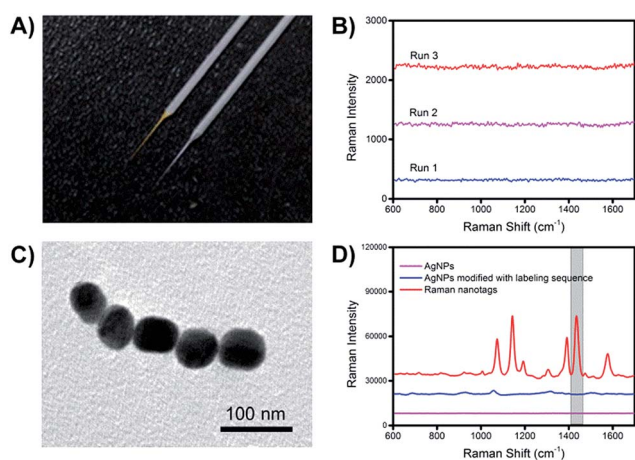
Fig. 3 (A) Photo of a bare starting microprobe (grey) and a final extraction microprobe (gold). (B) Raman spectra of the extraction sequence-functionalized microprobe. (C) Transmission electron microscopic (TEM) image of a Raman nanotag. (D) Raman spectra of bare AgNPs, AgNPs modified with only labelling sequence and Raman nanotags (AgNPs modified with labelling sequence and Raman reporter).
