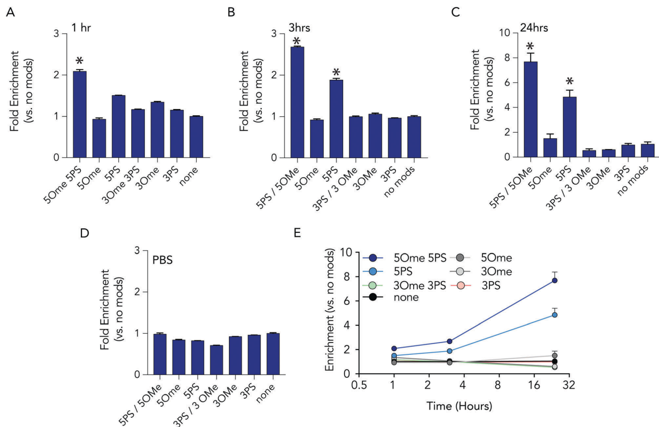
Fig. 3 Barcodes with 5 phosphorothioates and 5 2-O-methyl modifications exhibit increased stability in serum. Enrichment of each DNA barcode compared to barcodes with no modifications in 10% mouse serum at (A) 1 hours, (B) 3 hours, and (C) 24 hours. (D) As one control, we measured enrichment in PBS at 24 hours, and found no differences. (E) Enrichment of the top 2 barcodes increased over time.
