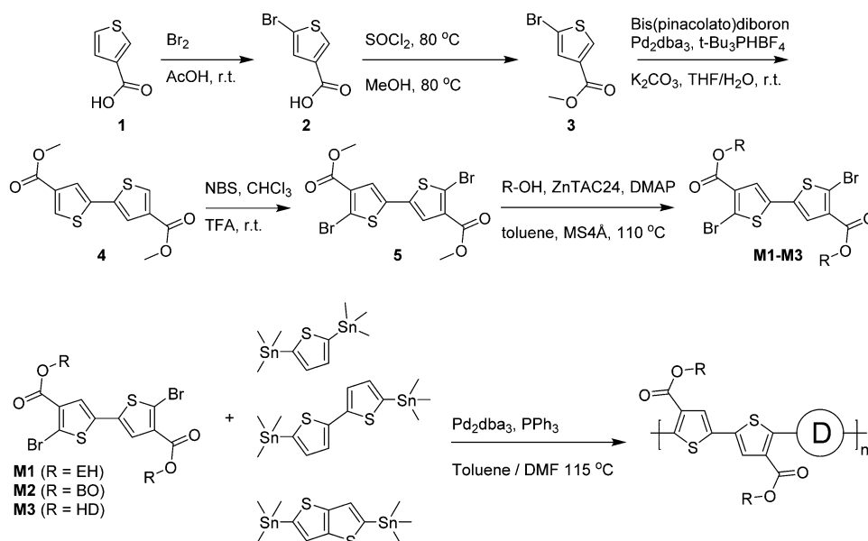
Scheme 1 Synthesis routes towards 2-ethylhexyl (EH), 2-butyloctyl (BO) and 2-hexyldodecyl (HD) substituted dicarboxylic ester bithiophene monomers (DCB) (top) and polymerization conditions for all nine combinations of monomers M1–M3 and thiophene (T), bithiophene (2T) and thienothiophene bistannyl monomers (TT) (bottom).
