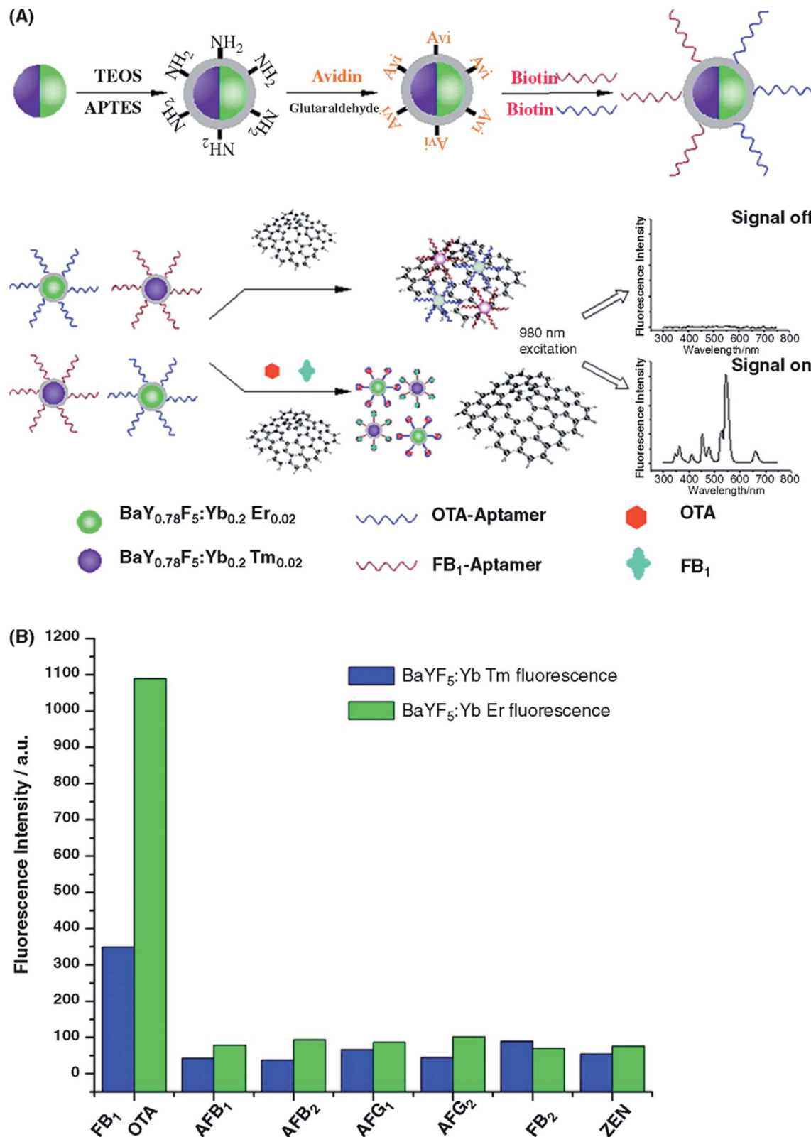
Fig. 35 (A) Schematic representation of the immobilization of ochratoxin A (OTA) aptamers and fumonisin B1 (FB1) aptamers and their multiplex upconversion FRET aptamer-UCNPs and GO for detecting OTA and FB1. (B) Fluorescence signal change for different mycotoxins at a concentration of 10 \text{ ng mL}^{-1} . FB1 and OTA show a significant increase in fluorescence intensity compared with other mycotoxin homologs, including AFB1, AFB2, AFG1, AFG2, fumonisin B2 (FB2) and zearalenone (ZEN), which are commonly found in foods. [Reprinted with permission from ref. 682, S. Wu, N. Duan, X. Ma, Y. Xia, H. Wang, Z. Wang and Q. Zhang, Multiplexed Fluorescence Resonance Energy Transfer Aptasensor between Upconversion Nanoparticles and Graphene Oxide for the Simultaneous Determination of Mycotoxins, Anal. Chem. , 2012, 84 , 6263–6270. Copyright© American Chemical Society.]
