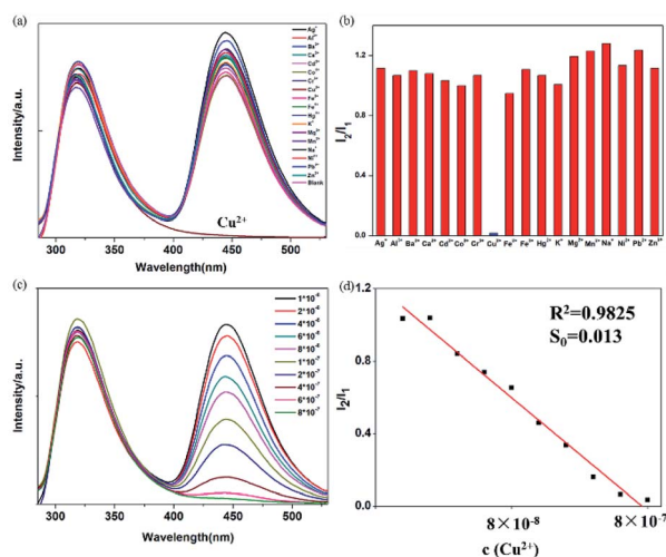
Fig. 6 (a) Fluorescence spectra of BBM-PMO-10 ( 5 \times 10^{-6} g \text{mL}^{-1} ) with different metal ions ( 10^{-6} M) in \text{THF}/\text{H}_2\text{O} = 3:7 (v/v); (b) fluorescence intensity ratio I_2/I_1 of BBM-PMO-10 ( 5 \times 10^{-6} g \text{mL}^{-1} ) with different metal ions ( 10^{-6} M) in \text{THF}/\text{H}_2\text{O} = 3:7 (v/v); (c) fluorescence spectra of BBM-PMO-10 in \text{THF}/\text{H}_2\text{O} = 3:7 (v/v) with different concentrations of \text{Cu}^{2+} ( 10^{-8} – 8 \times 10^{-7} M); (d) linear relationship between I_2/I_1 of BBM-PMO-10 ( 5 \times 10^{-6} g \text{mL}^{-1} ) and the concentration of \text{Cu}^{2+} in the solvent.
