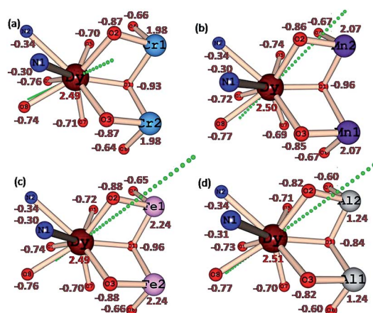
Fig. 8 Ab initio computed LoProp charges on the metal atoms and donor atoms of complexes (a) 1 {Cr 2 Dy 2 }, (b) 3 {Mn 2 Dy 2 }, (c) 5 {Fe 2 Dy 2 } and (d) 7 {Al 2 Dy 2 } (note: because of identical charges on the other half side, we have only shown here one side of the molecule).
