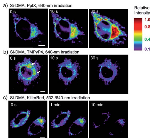
Fig. 12 Fluorescence microscopy images of HeLa cells treated with 18 and (a) 5-ALA induced protoporphyrin IX (PpIX), (b) tetrakis( N -methyl-4-pyridyl)porphyrin (TMPyP4), and (c) a lysosome marker (A647-dextran), and (c) mitochondrion-targeted KillerRed. (a and b) Cells were irradiated with a 640 nm laser to generate ^1\text{O}_2 and monitor the fluorescence induced by 18 simultaneously. (c) Two-color irradiation at 532 and 640 nm was used to excite 18 and KillerRed. Adapted with permission from ref. 41b. Copyright 2014 American Chemical Society.
