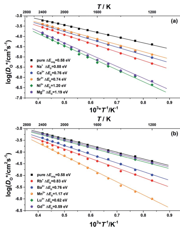
Fig. 3 Oxygen tracer diffusion coefficients ( D_O^* ) for various substituted, rhombohedral \text{BiFeO}_3 compositions obtained from MD simulations against inverse temperature: (a) data for substituent cations that should maximise D_O^* ; (b) data for substituent cations that should minimise D_O^* .
