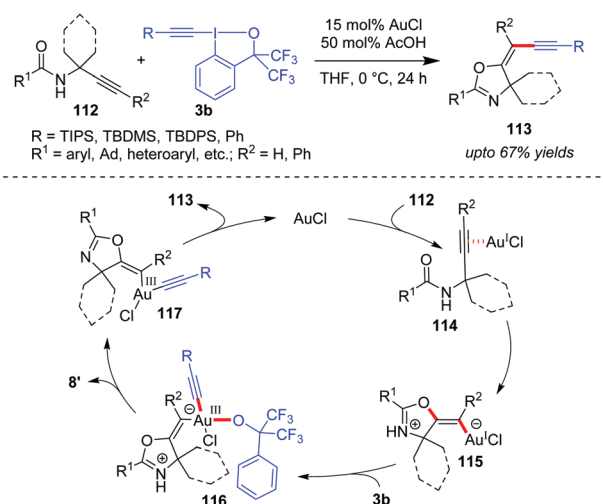
Scheme 18 Stereoselective domino cyclization/alkynylation of N -propargylcarboxamides.
