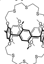
Pillar[5]-bis-trithiacrown (L)
