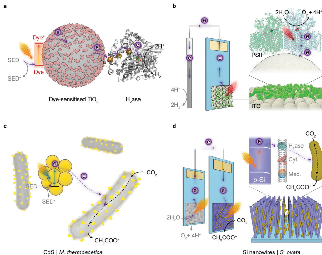
Fig. 5 Representative semi-artificial photosynthesis systems. (a) A colloidal system with dye-sensitised \text{TiO}_2 nanoparticles and \text{H}_2\text{ase} . 145 Under irradiation, the dye is excited and donates electrons to the conduction band of \text{TiO}_2 . The photoelectrons are then delivered to the catalytic centre of \text{H}_2\text{ase} for proton reduction via intraprotein electron relays. The oxidised dye is regenerated by extracting electrons from a sacrificial electron donor (SED). (b) An electrode system with a three-dimensional indium tin oxide (ITO) electrode and PSII. 102,120 PSII is wired by the porous ITO scaffold and photocatalyses water oxidation, aided by an applied potential. (c) A colloidal system with light absorbing CdS nanoparticles deposited on the \text{CO}_2 -reducing bacterium M. thermoacetica . 226 The excited CdS transfers photoelectrons to the bacterium, which generates reducing equivalents to produce acetate from \text{CO}_2 via the Wood–Ljungdahl pathway. The holes in CdS are quenched by the SED. (d) A hybrid tandem system with \text{TiO}_2 nanowires as the photoanode and p-Si nanowires integrated with acetogenic bacteria S. ovata as the photocathode. 248 When irradiated, the \text{TiO}_2 electrode oxidises water while p-Si nanowires generate photoelectrons that are delivered to the interfacing S. ovata via extracellular electron transfer pathways. S. ovata uses these electrons to reduce \text{CO}_2 into acetate through the Wood–Ljungdahl pathway.
