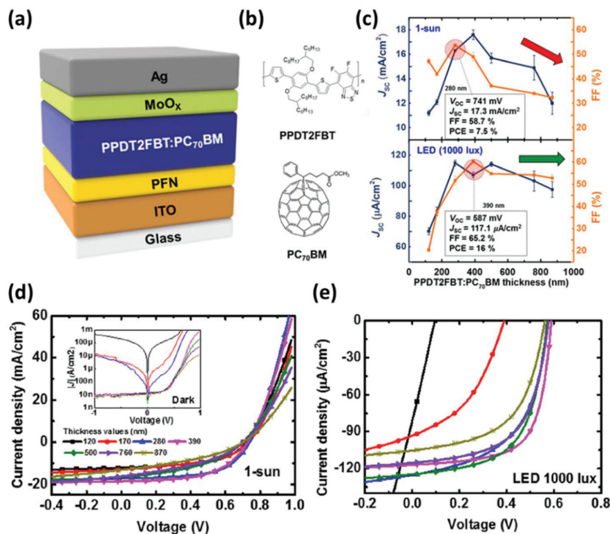
Fig. 5 Active layer thickness effect under 1 sun and LED illumination. (a) The device architecture and (b) molecular structures of PPDT2FBT and PC 70 BM. (c) Active layer thickness dependent J SC and FF under 1 sun and LED illumination. J–V characteristics with various photoactive layer thicknesses under (d) AM 1.5G and (e) LED (1000 lx) illumination. (Inset of (d): dark J–V curves.) Reproduced from ref. 47 with permission from Elsevier.
