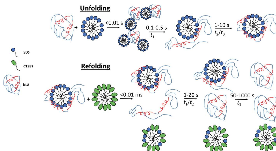
Fig. 8 Sketch showing the suggested unfolding and refolding scheme when bLG is unfolded with SDS and subsequently refolded with C 12 E 8 . Unfolding occurs in three steps with an initial clustering of SDS and protein within the deadtime of the experiment, followed by disaggregation of the complexes into individual SDS micelles with asymmetrically distributed protein, as seen by changes in Trp fluorescence, near-UV CD, and SAXS. In the last step, the protein is redistributed more symmetrically around the SDS micelle, as seen with changes in SAXS, near/far-UV CD, and Trp fluorescence. Refolding is somewhat more complex and slow and also involves three steps. Within the deadtime, a fraction of the protein dissociates from the surfactant micelles while the rest remains in complex, as observed by SAXS. Next, the unfolded protein is folded to a native state and finally the protein still in complex dissociates and refolds. \alpha -Helices are shown in red and two \alpha -helices represent a structure with native-like secondary structure, while three helices represent structures with increased \alpha -helical content. Note that for the refolding process there are additional changes in aggregation state of some of the species, which for simplicity are not indicated in the figure.
