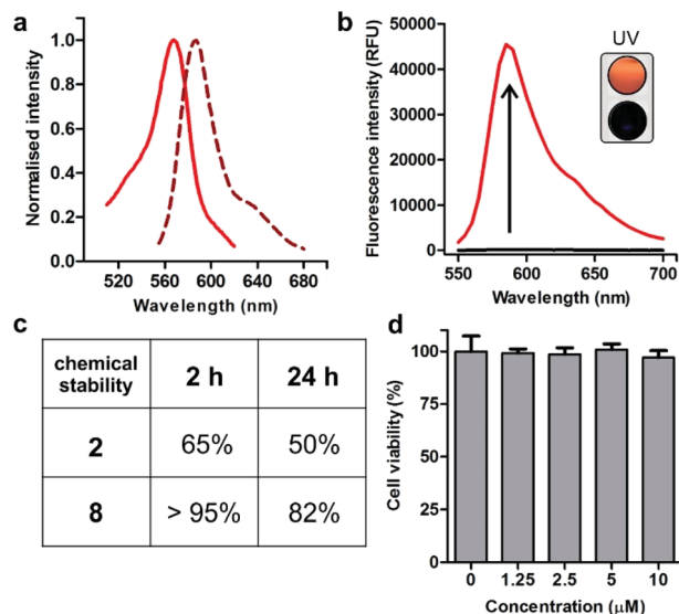
Fig. 2 (a) Absorbance and emission spectra of Trp(redBODIPY)-labelled peptide 8 (10 μM) in EtOH. Normalised absorbance (solid line) and fluorescence emission (dashed line, \lambda_{\text{exc}} : 520 nm). (b) Fluorogenic behaviour of cyclopeptide 8 (40 μM) in hydrophilic and hydrophobic media (70-fold). Peptide 8 was incubated in PBS (black) or in phosphatidylcholine liposome suspensions (red, \lambda_{\text{exc}} : 520 nm). (Inset) Naked eye pictograms of both solutions under a hand-held UV lamp using 365 nm excitation. (c) Stability of peptides in a protease cocktail by HPLC monitoring. (d) Viability of HeLa cells after incubation with different concentrations of peptide 8 . Values are presented as means \pm s.d. ( n = 4 ). Non-significant differences ( p > 0.05 ) were observed between the untreated control and any of the treatments.
