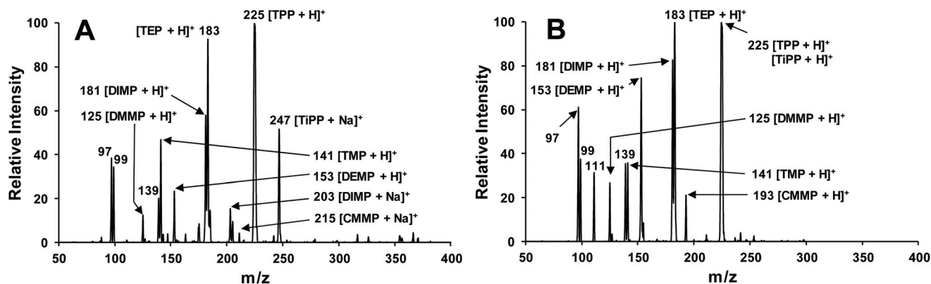
Fig. 3 3D-PCSI-MS collected on the portable Al-MS from a mixture of DMMP, TMP, DEM, DIMP, TEP, CMMP, TPP, and TiPP (all at 5 ppm each) in sand. Spectra (A) collected at 1 min of analysis time yield both protonated and sodiated adducts for some target CWA simulants, where spectra (B) from ~7 min predominately show only the protonated forms, as salt leaves the sand matrix.
