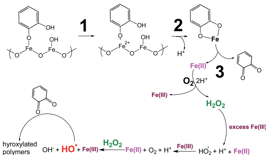
Scheme 5 A three-step mechanism for abiotic oxidative polymerization of catechol on the surface of iron oxide proposed by Colarieti et al. 254 and Larson and Hufnagel. 217 The different colors are used to highlight the oxidation state of the iron in the respective step. The larger size of OH and H 2 O 2 is used to highlight the reactive oxygen species generated in the reaction. Reproduced from ref. 206 with permission from the American Chemical Society, © 2020.
