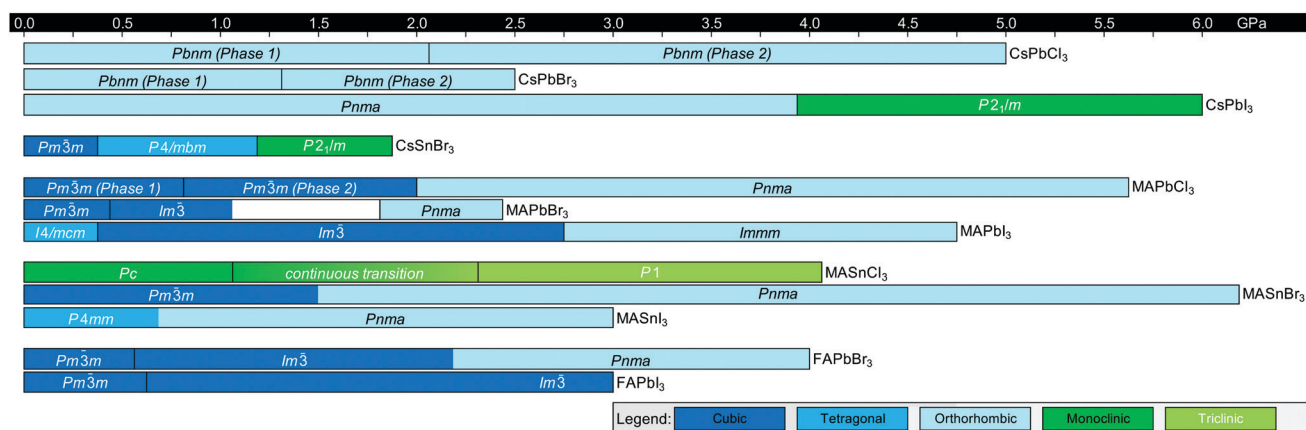
Promisingly, recent reports have found that some pressure-induced changes can be retained upon cycling back to ambient pressure. For \text{FAPbI}_3 exposed to pressures of 7.1 GPa, it was found that unit cell parameters at ambient pressure after compression were smaller compared to before compression, as evidenced by a shift in diffraction peaks to higher 2-theta values. 176 This structural change resulted in a narrower bandgap of previously compressed versus uncompressed \text{FAPbI}_3 . Recently, quenching \text{MAPbI}_3 from a high pressure state was found to result in retention of bandgap reduction upon
