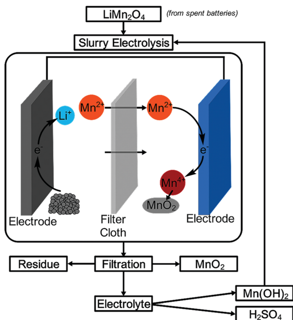
Scheme 1 Device operation for the recovery of manganese from spent batteries using slurry electrolysis.
