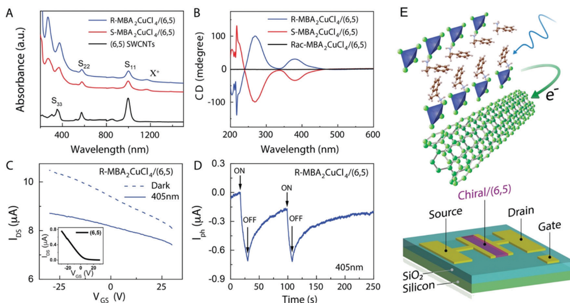
Fig. 13 (A) UV-Vis-NIR absorption spectra of SWCNT, R- and S-MBA 2 CuCl 4 /SWCNT. (B) CD signals of R- and S-MBA 2 CuCl 4 /(6,5) SWCNT and (rac\text{-MBA})_2\text{CuCl}_4/(6,5) SWCNT. (C) A comparison of the effects of dark and photoresponse conditions on the FET transfer curve. (D) The photocurrent response of (R\text{-MBA})_2\text{CuCl}_4/\text{SWCNT} over time. (E) A schematic description of a three-terminal FET device. Reprinted with permission. 104 Copyright 2021, American Chemical Society.
