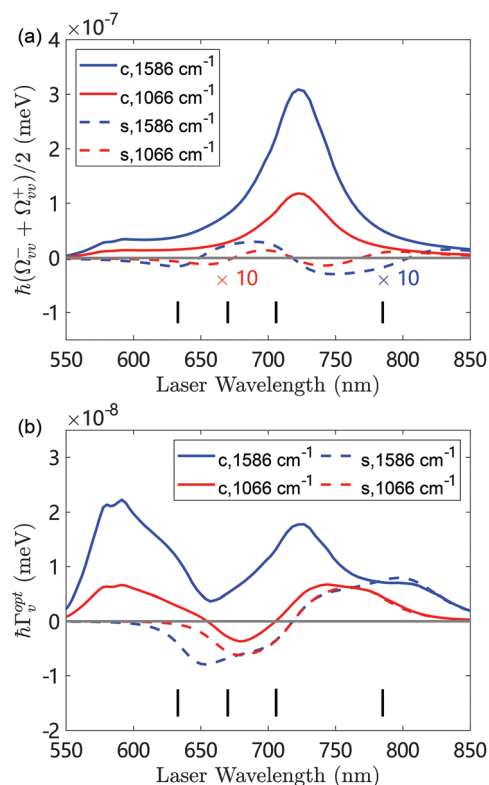
Fig. 5 (a) Vibrational frequency shift (\Omega_{\text{vv}}^+ + \Omega_{\text{vv}}^-)/2 and (b) effective optomechanical damping rate \Gamma_{\text{vv}}^{\text{opt}} = \Gamma_{\text{vv}}^- - \Gamma_{\text{vv}}^+ as a function of the laser wavelength for the 1586\text{ cm}^{-1} vibrational mode (blue lines) and the 1066\text{ cm}^{-1} vibrational mode (red lines). The solid and dashed lines are the results from the continuum-field model (labeled as “c”) and the single-mode model (labeled as “s”), respectively. The vertical lines indicate wavelengths at 633 nm, 670 nm, 705.9 nm and 785 nm used for later simulations. The laser intensity is 1\text{ }\mu\text{W }\mu\text{m}^{-2} and other parameters are specified in the text.
