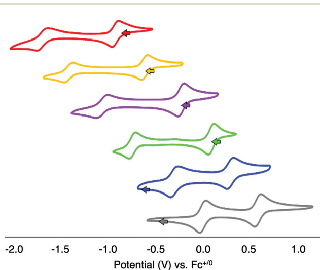
Fig. 6 Cyclic voltammograms of complexes 1 (red, top), 2 (orange), 1 -(OMe) (purple), 2 -(OMe) (green), 1 -(OMe) 2 (blue), and 2 -(OMe) 2 (gray, bottom). All voltammograms were collected using 1 mM solutions of the complexes in acetonitrile with 0.1 M [\text{t}^{\text{Bu}}_4\text{N}][\text{PF}_6] as the supporting electrolyte at a scan rate of 200 \text{mV s}^{-1} .
