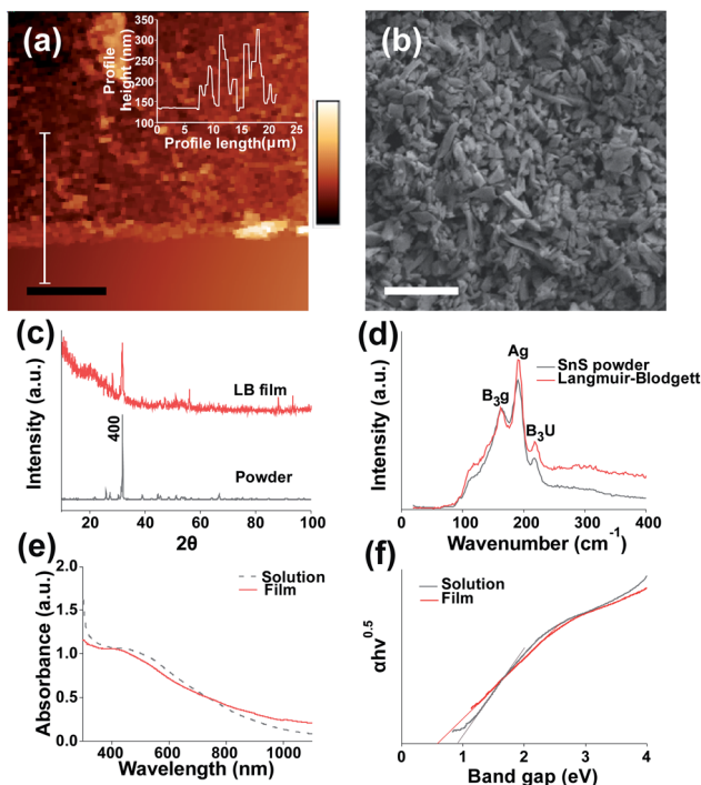
Fig. 1 Structural characterisation of SnS nanosheet thin films assembled by the Langmuir-Blodgett method. (a) AFM image of LB assembled SnS film edge. Inset film profile, scale bar = 10 μm. (b) SEM image of LB assembled film on Si/SiO 2 at 3 kV using secondary electron imaging, scale bar = 1 μm. (c) XRD pattern of coated film and bulk SnS powder, (additional peaks labelled in Fig. S2†). (d) Raman spectra and for bulk and Langmuir-Blodgett assembled SnS nanosheets. (e) UV-Vis spectra of SnS suspension and deposited SnS film on glass (f) Tauc plot of SnS solution and film.
