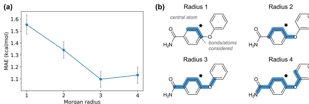
Fig. 9 (a) Mean absolute error for \text{GPR}_{\text{M3/2}} as a function of Morgan fingerprint radius. (b) Atoms and bonds considered by Morgan fingerprints of different radius. A radius of radius three or more is needed to capture the effect from groups in the para position of the aromatic ring.
