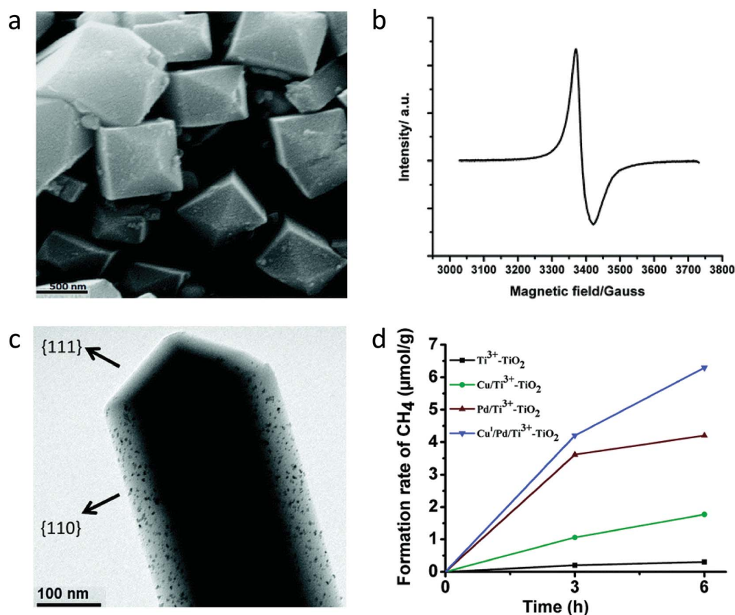
Fig. 19 (a) SEM image of the \text{Ti}^{3+}\text{-TiO}_2 sample and (b) EPR spectra of the \text{Ti}^{3+}\text{-TiO}_2 sample recorded at 100 K, (c) TEM images of the \text{Cu/Pd/Ti}^{3+}\text{-TiO}_2 sample, and (d) comparison of photocatalytic \text{CO}_2 conversion using different samples (reproduced from ref. 73 with permission from the Royal Society of Chemistry, copyright 2015).
