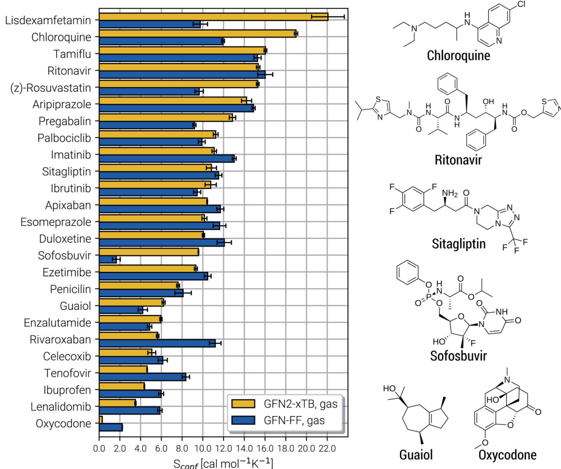
Fig. 8 Calculated S_{conf} values for a set of 25 clinical drug molecules at the GFN2-xTB and GFN-FF levels of theory sorted according to increasing value. Averaged values (shown as horizontal bars) and their standard deviations (shown as errors) have been determined by multiple executions of the above described algorithm, as described in the text below. On the right side Lewis structures of some of the molecules are shown (see the ESI† for all molecules).
