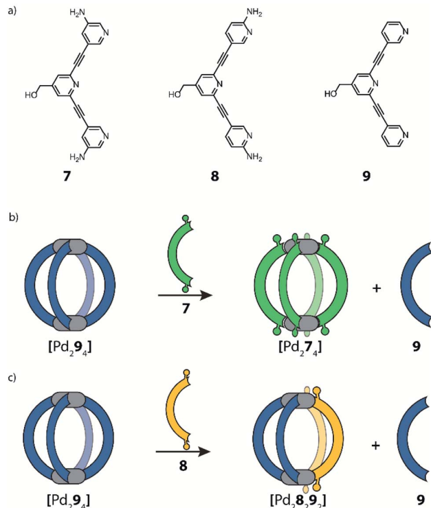
Fig. 6 (a) Banana-shaped ligands bearing amino substituents at the pyridyl donor groups; (b) addition of ligand 7 to [Pd_2.9_4] leads to complete displacement of 9; (c) formation of heteroleptic cage cis-[Pd_2.8.9_2] can be achieved by partial ligand displacement under kinetic control.
