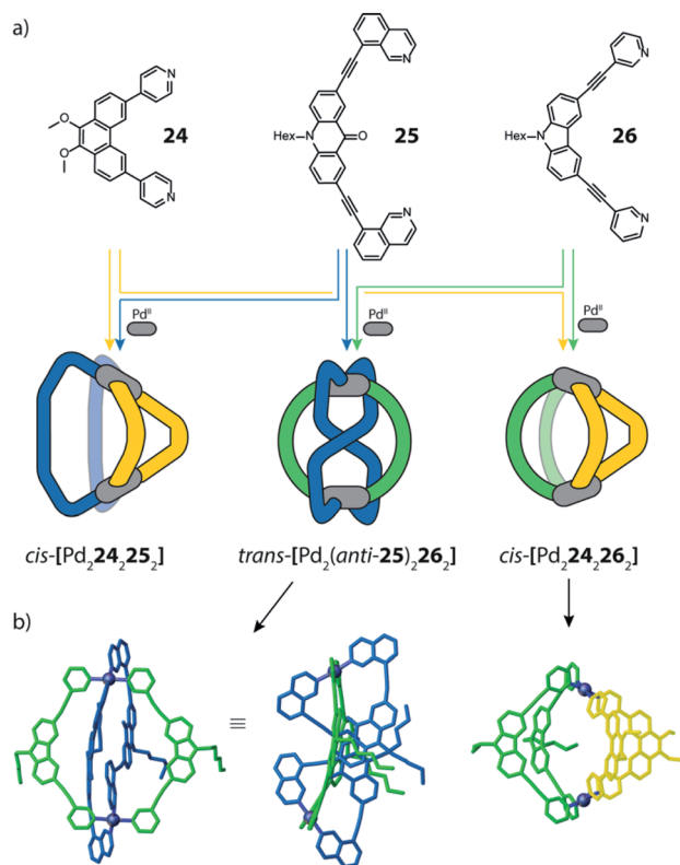
Fig. 11 (a) Self-assembly of cis - and trans -heteroleptic cages using shape complementarity; (b) single crystal X-ray structures of trans-[Pd_2(anti-25)_226_2] and cis-[Pd_22426_2] .
