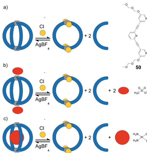
Fig. 21 (a) Reversible switch between [Pd_250_4] and [Pd_250_2Cl_4] in acetonitrile or DMF upon addition/sequestration of chloride; (b) mesylate guest binds exohedrally to [Pd_250_4] and is released upon addition of chloride; (c) cis-platin binds in the cavity of [Pd_250_4] . Formation of the ring releases the guest.
