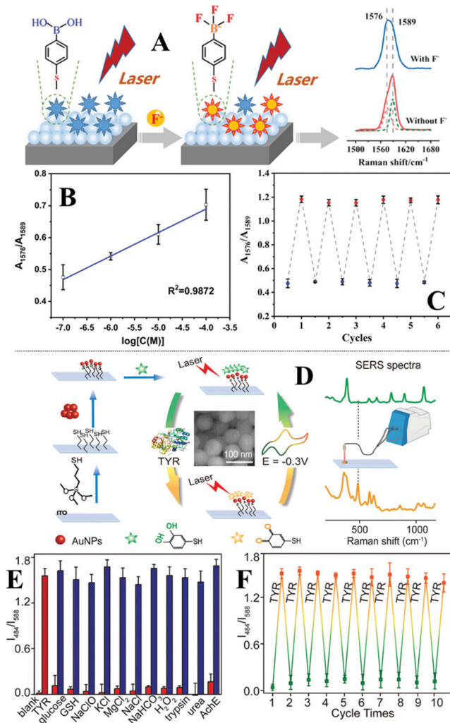
Fig. 20 (A) Schematic illustration of the working principles of the pH-reversible F^- sensor; (B) plot showing the average area ratio between the SERS peak at 1576\text{ cm}^{-1} and 1589\text{ cm}^{-1} as a function of the log concentration of F^- ; (C) plot showing the SERS activity of the sensor after 6 cycles of regeneration; (D) schematic illustrations of the fabrication of the electro-reversible tyrosinase sensor. Inset shows a SEM image of the enhancing Au nanoparticles on the surface of the sensor; (E) bar chart showing the ratio value between the SERS intensity of the vibration bands at 484\text{ cm}^{-1} and 588\text{ cm}^{-1} as a function of sample type. The red histograms correspond to the signals obtained from blank reference samples and pure samples of the chemicals labelled below. The blue histograms correspond to samples containing a mixture of tyrosinase and the chemicals labelled below. The error bars represent the standard deviation calculated from 3 independent measurements; (F) plot showing the SERS activity of the sensor after 10 cycles of electro-regeneration. Panel (A–C) reproduced with permission from ref. 272, copyright 2019 American Chemical Society. Panel (D–F) reproduced with permission from ref. 273, copyright 2019 American Chemical Society.
