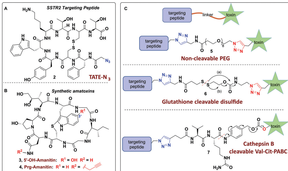
Fig. 2 (A) Chemical structures of sstr2 targeting agent octreotate (TATE-N 3 , 2 ); (B) synthetic bioactive amatoxins 3 and 4 ; (C) three bioconjugates 5 – 7 synthesized in this study. Highlighted in blue and red are conjugation sites; (a) and (b) show two proposed pathways for self-immolative drug release of bio-reducible linker conjugate 6 .
