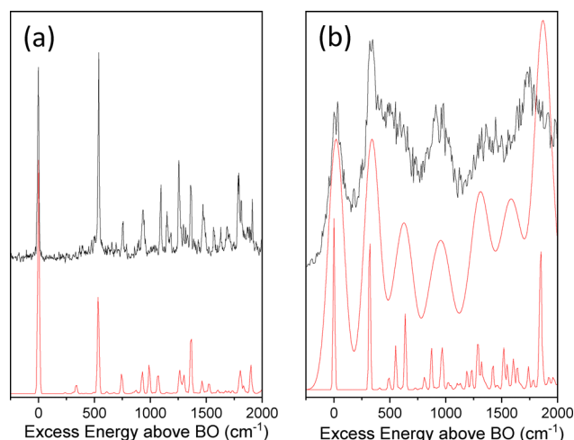
Fig. 5 Comparison between the experimental and FC simulations of (a) the D_0-D_4 transition of C_1^{*+} and (b) the D_0-D_3 transition of C_4^{*+} . Calculated frequencies (UCAM-B3LYP/aug-cc-pVDZ) scaled by 0.95. BO is for "Band Origin".
