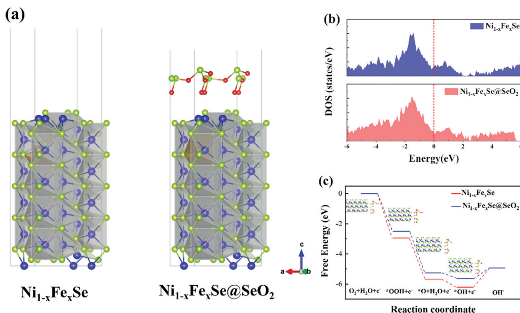
Fig. 5 Theoretical calculations of \text{Ni}_{1-x}\text{Fe}_x\text{Se} and \text{Ni}_{1-x}\text{Fe}_x\text{Se@SeO}_2 electrocatalysts. (a) Crystal structures, (b) calculated DOS, (c) free energy diagram for the OER over four optimized adsorption geometry of \text{O}_2 , ^*\text{OOH} , ^*\text{O} , and ^*\text{OH} .
