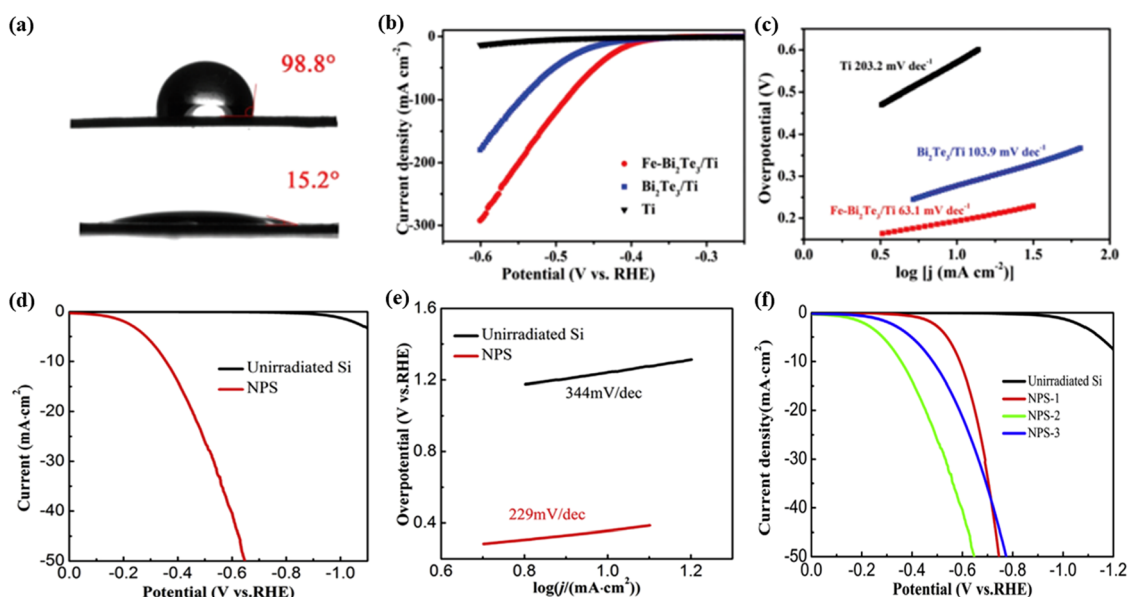
Fig. 10 (a) Contact angles of Bi 2 Te 3 /Ti (top) and Fe-Bi 2 Te 3 /Ti (bottom), respectively. (b) LSV curves of the Ti plate, Bi 2 Te 3 /Ti and Fe-Bi 2 Te 3 /Ti at a scan rate of 5 \text{mV s}^{-1} . (c) The corresponding Tafel plots. Reproduced with permission from ref. 35. Copyright 2020, Royal Society of Chemistry. (d) Polarization curves of the nanoporous and non-irradiated Si. (e) Tafel slopes derived from the polarization curves. (f) The polarization curves for the fluences of NPS-1, NPS-2 and NPS-3. Reproduced with permission from ref. 67. Copyright 2018, Elsevier.
