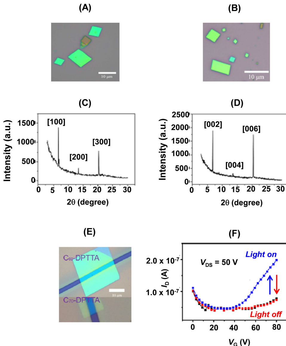
Fig. 15 Optical micrographs of self-assembled 22a -C 60 (A) and 22a -C 70 (B); XRD patterns of 22a -C 60 (C) and 22a -C 70 (D); (E) optical image of the single crystal BGTC devices; (F) phototransistor responses of the 22a -C 70 microcrystal based transistor under light irradiation. Reproduced with permission from ref. 32. Copyright 2013, The American Chemical Society.
