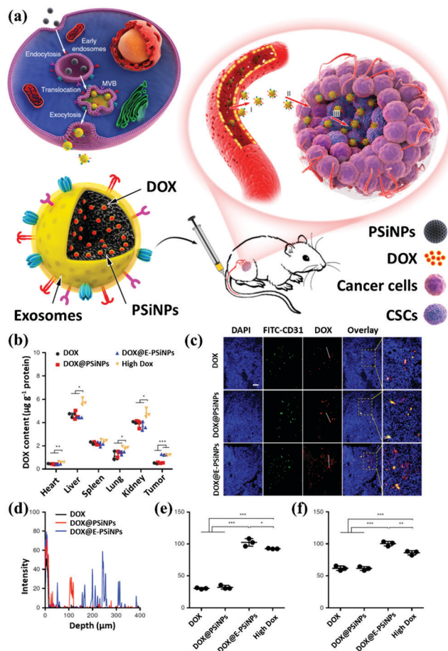
Fig. 7 Schematic illustration of E-PSiNPs as drug carriers for targeted cancer chemotherapy. (a) Schematic illustration of the preparation of DOX@E-PSiNPs. DOX@PSiNPs are endocytosed into cancer cells after incubation and localized in multivesicular bodies (MVBs) and autophagosomes. After MVBs or amphisomes fuse with the cell membrane, DOX@E-PSiNPs are exocytosed into extracellular space. (b) Schematics showing how DOX@E-PSiNPs efficiently target tumor cells after intravenous injection into tumor-bearing mice. (c) The confocal images and (d) signal quantification of DOX@E-PSiNPs accumulation. The DOX accumulation under (e) neutral and (f) low pH values. Reproduced with permission. 78 Copyright 2019, Springer Nature Limited.
