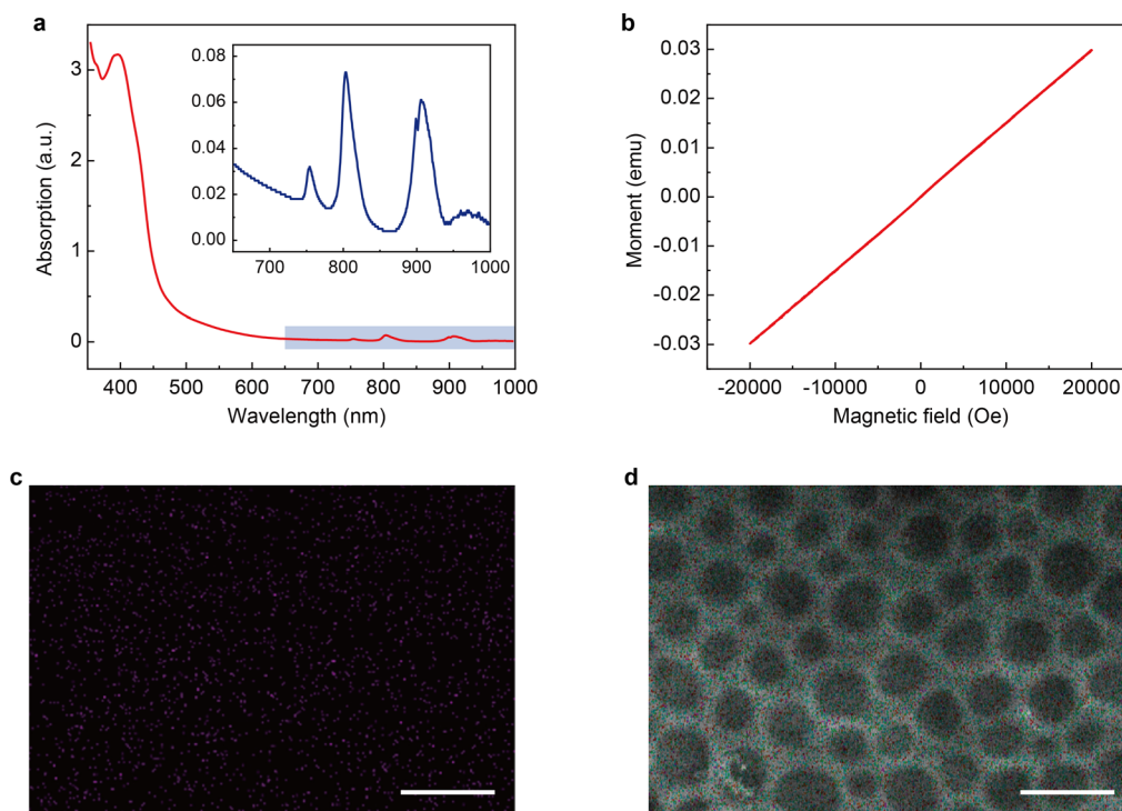
Fig. 3 Characterization of magnetic polyionic liquid micropores and the magnetic ionic liquid. (a) UV-Vis spectrum of the magnetic ionic liquid [HS-C 10 mim] [Dy(NO 3 ) 4 ]. The inset shows the magnified image of the 650–1000 nm region. (b) Magnetization curve of [HS-C 10 mim] [Dy(NO 3 ) 4 ]. The measurement was performed at room temperature. (c) Dy elemental distribution and (d) EDS results of magnetic polyionic liquid micropores. The scale bars in (c) and (d) are 5 \mu m.
