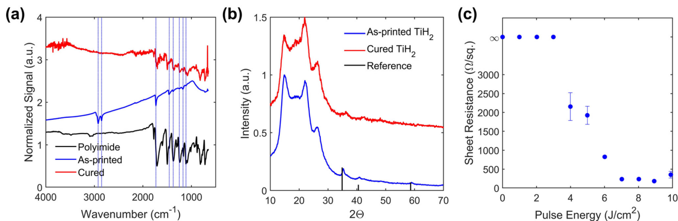
Fig. 6 Analysis of the photonic curing process, including (a) FTIR, (b) pXRD, and (c) electrical sheet resistance for \text{TiH}_2 films before and after IPL curing. Reference pXRD peaks in (b) correspond to PDF 00-025-0982.
