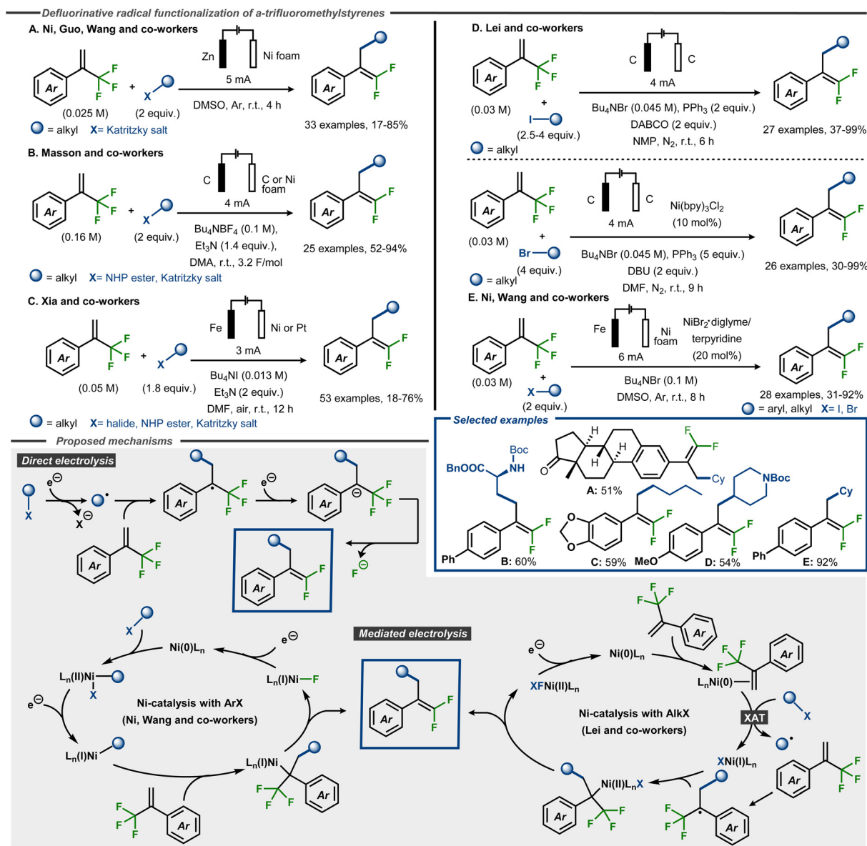
Fig. 18 Electroreductive formation of \gamma -functionalized gem -difluorostyrenes from \alpha -trifluoromethyl styrenes and radical precursors. 64–68
