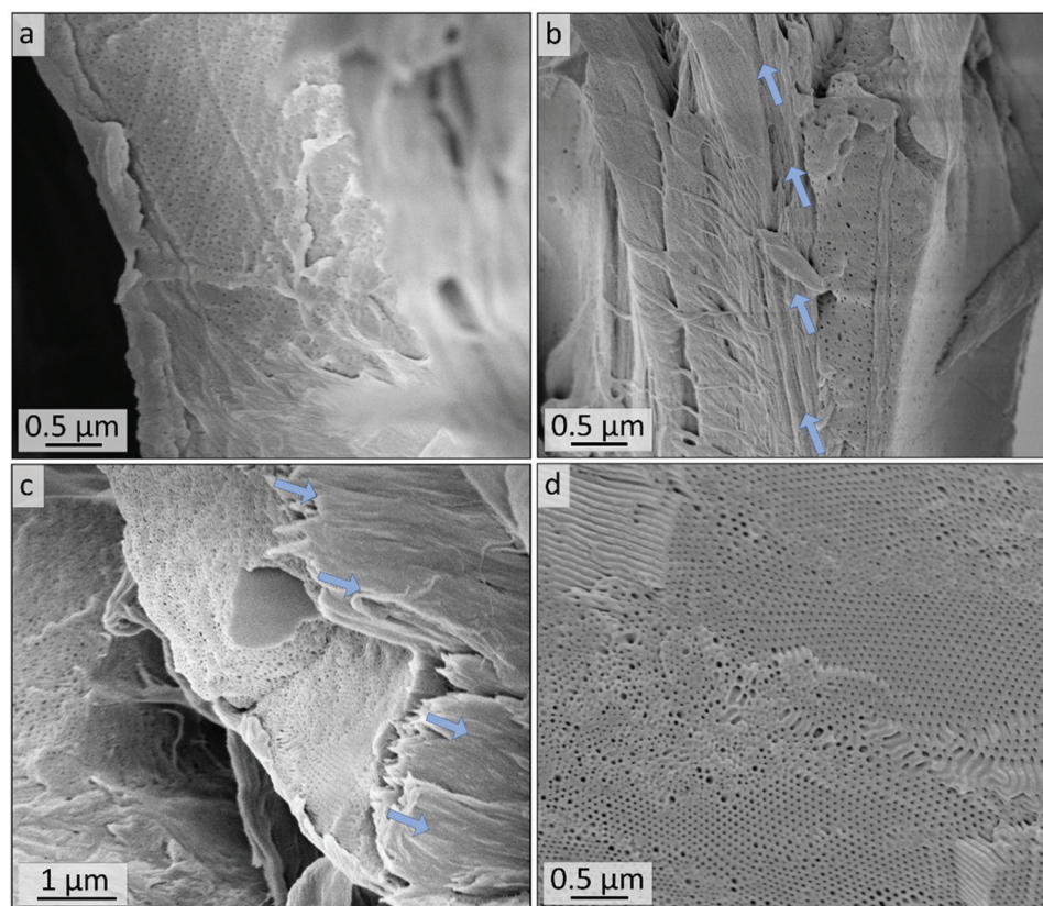
Fig. 9 SEM analysis of the (a and b) cross-sections of untreated and (c and d) ozone treated composite material (sample Cs10) using \text{PI}_{35}\text{-b-P2VP}_{65}^{186} on Munktell cellulose-based filter discs. Blue arrows indicate cellulose fibers.
