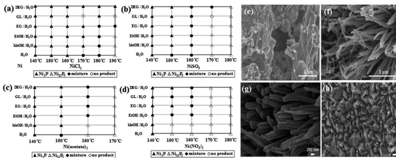
Fig. 4 Synthesis of nickel phosphides via the solvothermal method with different nickel precursors: (a) NiCl 2 ·6H 2 O, (b) NiSO 4 ·6H 2 O, (c) Ni(acetate) 2 ·4H 2 O and (d) Ni(NO 3 ) 2 ·6H 2 O (mixed solvents are a mixture with equal volume ratio and MeOH, EtOH, EG, GL, and DEG stand for methanol, ethanol, ethylene glycol, glycerol and diethylene glycol, respectively). 43 SEM images of NiCo 2 S 4 : (e) without using nickel foam and (f) with use of nickel foam (reproduced from ref. 66 with permission from Wiley, Copyright 2016). SEM images of (g) V-doped Ni 3 S 2 using Na 3 VO 4 ·12H 2 O and (h) Ni 3 S 2 (reproduced from ref. 68 with permission from the American Chemical Society, Copyright 2017).
