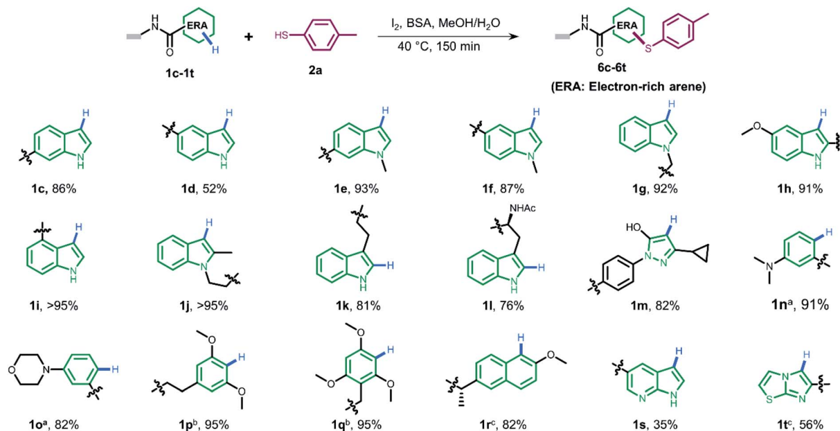
Fig. 3 The substrate scope of different DNA-conjugated ERAs in the sulfenylation reaction and the corresponding conversions. Deviation from above reaction condition a reaction time is 6 h. b \text{I}_2 (400 nmol, 13.3 mM). c \text{I}_2 (800 nmol, 26.7 mM).
