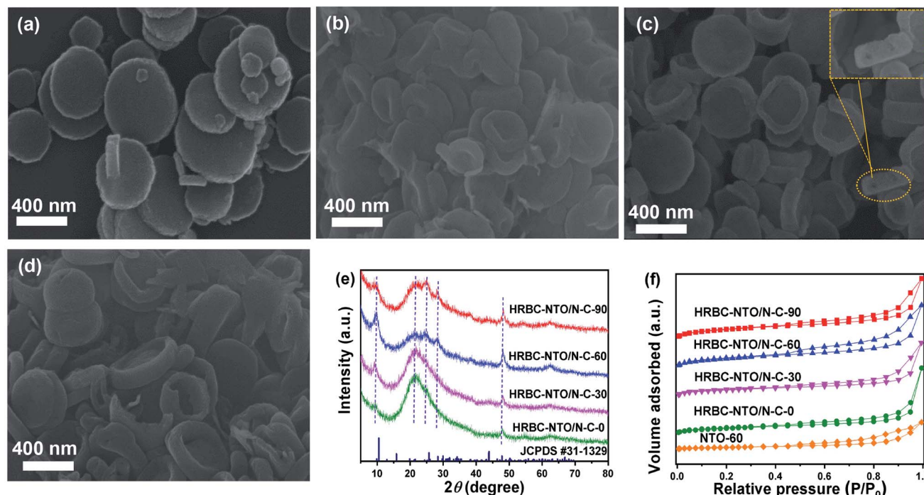
Fig. 3 SEM images of (a) HRBC-NTO/N-C-0, (b) HRBC-NTO/N-C-30, (c) HRBC-NTO/N-C-60, and (d) HRBC-NTO/N-C-90. (e) XRD patterns of HRBC-NTO/N-C- x . (f) N 2 sorption isotherms of HRBC-NTO/N-C- x and NTO-60.
