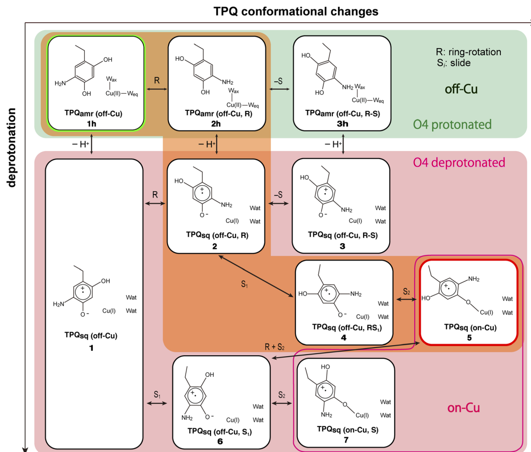
Fig. 4 A comprehensive view of the intermediate states on which the present work is focused for the TPQ amer to TPQ sq transition. The letter "h" added in the labeling as in 1h–3h stands for the protonated state on O4-TPQ. The orange background highlights the main reaction pathway, whereas the green background refers to the O4-TPQ protonated state, and the red one refers to the deprotonated one.
