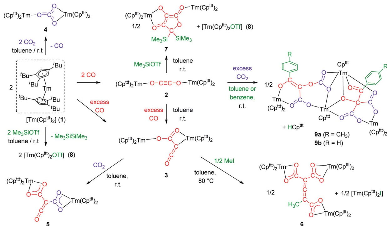
Scheme 5 Summary scheme of all the reactivity described in this study starting from [\text{Tm}(\text{Cp}^{\text{tBu}})_2] (1).
