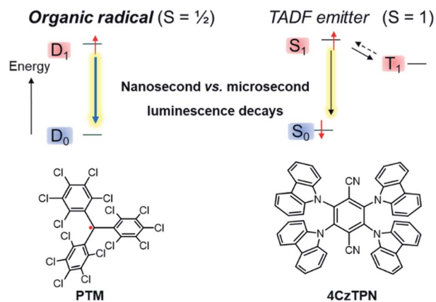
Fig. 2 Comparison of the emission process of the organic radical emitter per -chlorotriphenylmethyl PTM (left) and the TADF emitter 2,3,5,6-tetra(9 H -carbazol-9-yl)terephthalonitrile, 4CzTPN (right). 44
