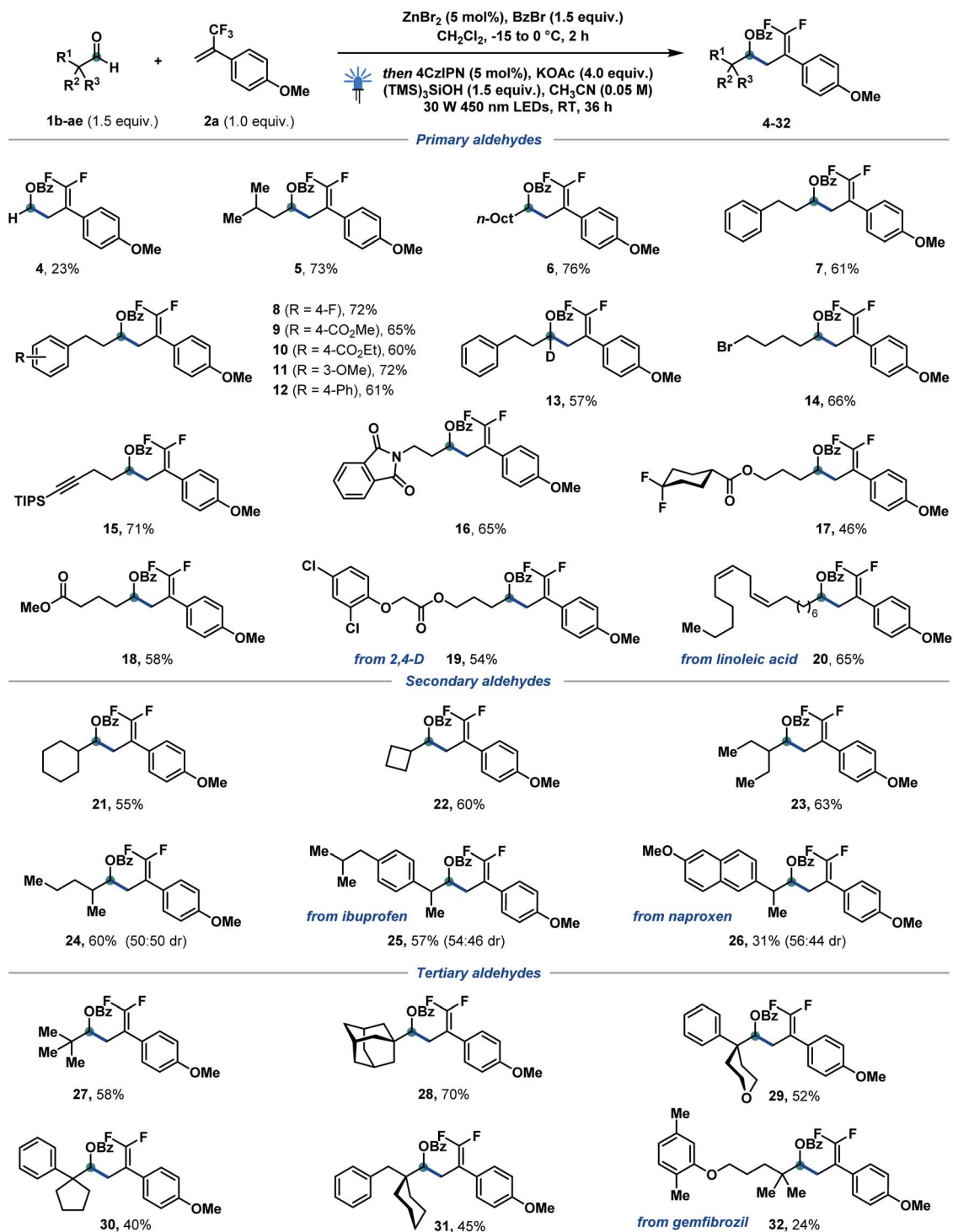
Scheme 2 Reaction scope of \alpha -primary, -secondary and -tertiary aldehydes. Reaction conditions: 1b–1ae (0.3 mmol, 1.5 equiv.), benzoyl bromide (0.3 mmol, 1.5 equiv.), \text{ZnBr}_2 (0.01 mmol, 5 mol%), \text{CH}_2\text{Cl}_2 (1 M), -15 to 0 °C, 2 h, then 2a (0.2 mmol, 1.0 equiv.), 4CzIPN (0.01 mmol, 5 mol%), KOAc (0.8 mmol, 4.0 equiv.), (\text{TMS})_3\text{SiOH} (0.3 mmol, 1.5 equiv.), MeCN (0.05 M), 30 W 450 nm LEDs, RT, 36 h. For experimental details, see the ESI.†
