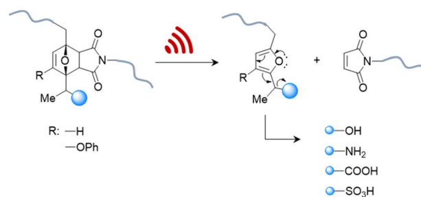
Fig. 4 US-induced cargo release from 2-furlycarbinol mechanophore via retro Diels-Alder reaction followed by fragmentation cascade. 87 The cargo scope includes alcohols (aryl/alkyl), amines (aryl/alkyl), carboxylic acids, and sulfonic acids.
