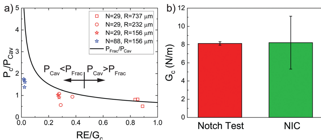
Fig. 4 (a) Plot of the experimentally observed critical expansion pressure P_c normalized by P_{Cav} against RE/G_c . The black line represents the point at which fracture is predicted to occur. (b) Plot showing the comparison between G_c measured with notch tests by Barney et al. 16 and measured with NIC in this work when RE/G_c \approx 0.84 .
