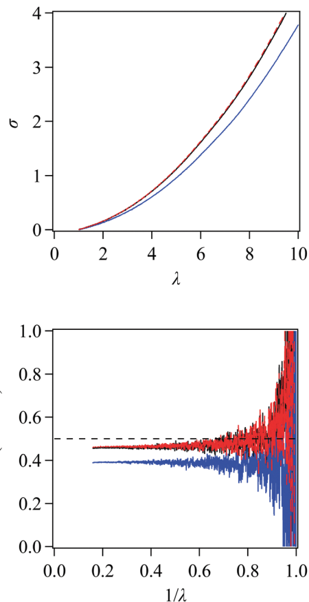
Fig. 7 Stress–strain relation under uniaxial stretch with a constant stretching rate for s2020 (red broken), 2a2-3802 (black solid), and Rnd (blue solid). The broken horizontal line indicates a value of 0.5.
