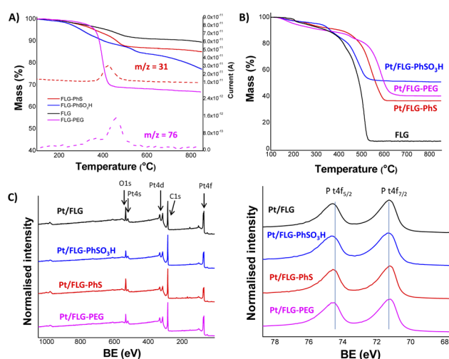
Fig. 1 Characterisation of functionalised graphene samples. (A) TGA-MS under \text{N}_2 of functionalised graphene samples. Phenyl and PEG fragments m/z = 76 ( \text{C}_6\text{H}_4^+ ) and m/z = 31 ( \text{CH}_3\text{O}^+ ), respectively. (B) TGA under air of platinum supported graphene samples. (C) XPS spectra of platinum supported graphene samples (left panel) and platinum Pt 4f component (right panel).
