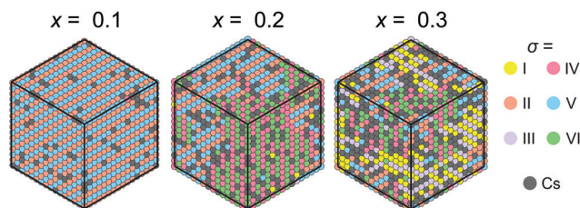
Fig. 7 Snapshots of simulations of our model for different \text{Cs}^+ ion concentrations. The FA cation states are represented in the \sigma -representations. Simulations are performed by starting from the disordered phase and gradually lowering the temperature significantly below T_0 . A multidomain structure is observed at the higher mixing levels. Simulation parameters: \varepsilon_1 = 21 meV, \varepsilon_2 = 12.6 meV, \varepsilon_{\text{CS}} = 31.5 meV, L = 16 .
